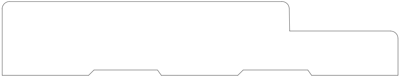
JAMB 46632 1 1/4" X 6 5/8"
