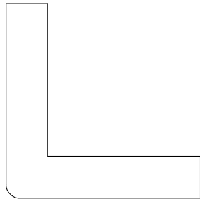
OUTSIDE CORNER 917518 1 3/4" X 1 3/4"
