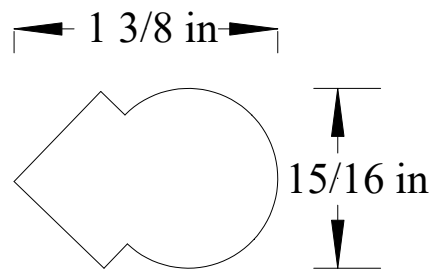
PENCIL MOULD 913817 15/16" X 1 3/8"
