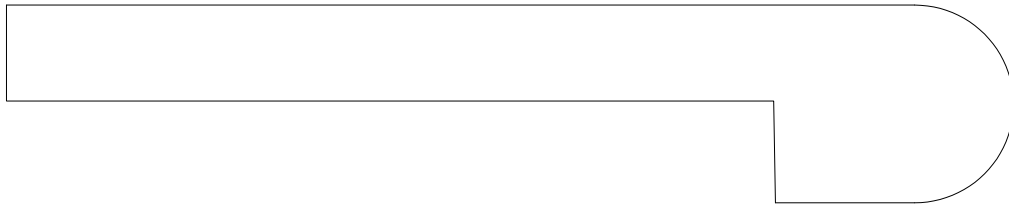
LANDING TREAD 952518 1 1/16" x 5 1/4"
