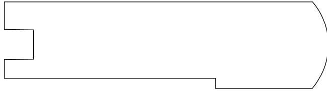
LANDING TREAD 93131 13/16" X 3 1/8"
