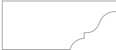
WAINSCOT CAP 925021 1 1/16" X 2 1/2"
