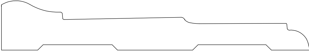
BASE 25008 13/16" X 5"
