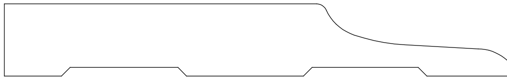
BASE 252519 3/4" X 5 1/4"
