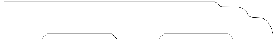
BASE 245027 5/8" X 4 1/2"
