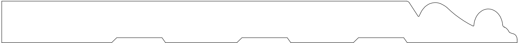
BASE 29253 3/4" X 9 1/4"
