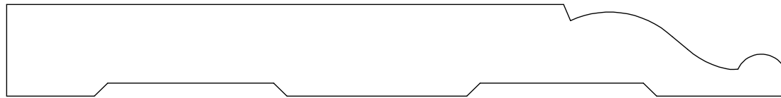
BASE 252513 5/8" X 5 1/4"
