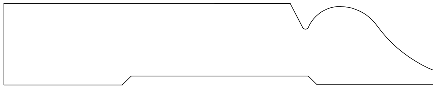
BASE 245019 7/8" X 4 1/2"
