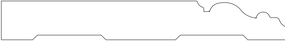
BASE 250010 11/16" X 5"
