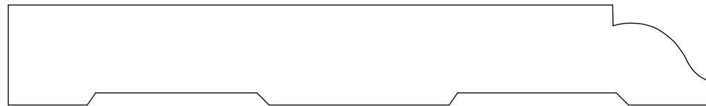
BASE 24881 11/16" X 4 7/8"
