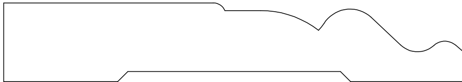
BASE 24006 11/16" X 4"
