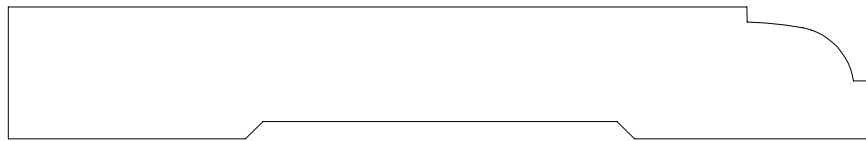
BASE 245032 11/16" X 4 1/2"
