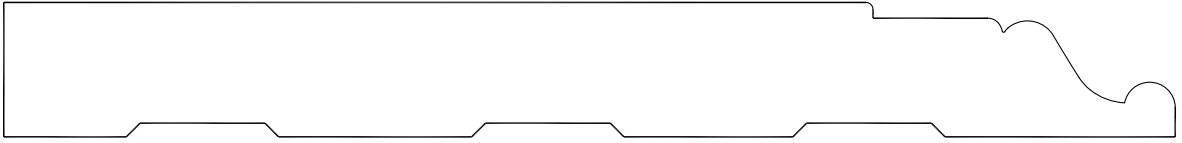
BASE 2763 7/8" X 7 5/8"
