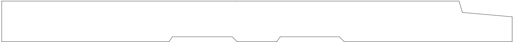
BASE 29252 3/4" X 9 1/4"
