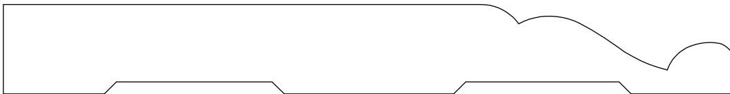
BASE 25255 5/8" X 5 1/4"
